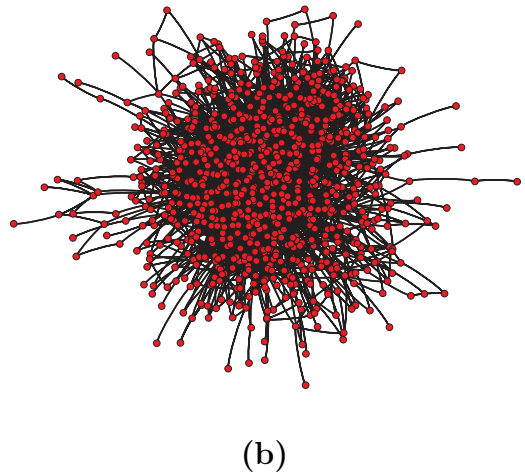
Figure 5.2. (a) Graph theoretic representation of a reaction in a metabolic network. (b) The complete E. coli metabolic network.
