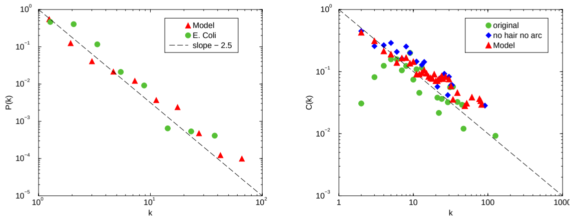
Figure 6.6. Log-binned distributions of the node's degree P(k) and clustering coefficient C(k) of the best fitting model and the metabolic network of E. coli .
