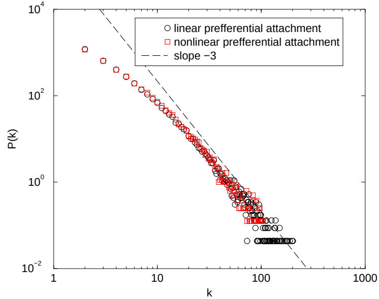
Figure 3.8. Connectivity distribution generated by the numerical simulations for linear ( \nu = 1 ) and nonlinear ( \nu = 0.75 ) preferential attachment ( N_{max} = 3500 , a = 0.0005 , \beta = 1 and b = 2 ).
