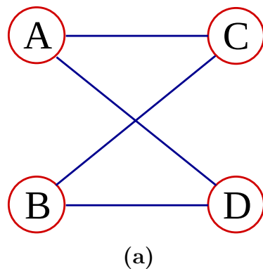
Figure 5.2. (a) Graph theoretic representation of a reaction in a metabolic network. (b) The complete E. coli metabolic network.
