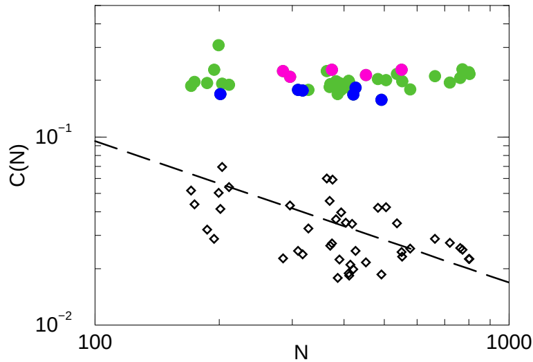
Figure 5.3. The average clustering coefficient for 43 organisms [101] is shown as a function of the number of substrates N present in each of them. Species belonging to archaea (purple), bacteria (green), and eukaryotes (blue) are shown. The dashed line indicates the dependence of the clustering coefficient on the network size for a module-free scale free network, and the diamonds denote C for a scale free network with the same parameters ( N and number of links) as observed in the 43 organisms.
