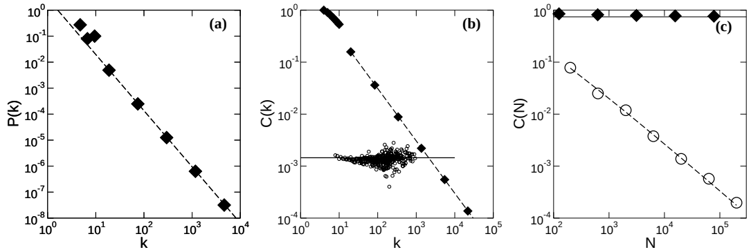
Figure 4.4. Scaling properties of the hierarchical model ( N = 5^7 ). (a) The numerically determined degree distribution. The asymptotic scaling, with slope \gamma - 1 = \ln 5 / \ln 4 , is shown as a dashed line. (b) The C(k) curve for the model, demonstrating that it follows equation (4.8). The open circles show C(k) for a scale free model [20] of the same size, illustrating that it does not have a hierarchical architecture. (c) The dependence of the clustering coefficient, C , on the size of the network N . While for the hierarchical model C is independent of N ( \blacklozenge ), for the scale free model C(N) decreases rapidly ( \circ ).
