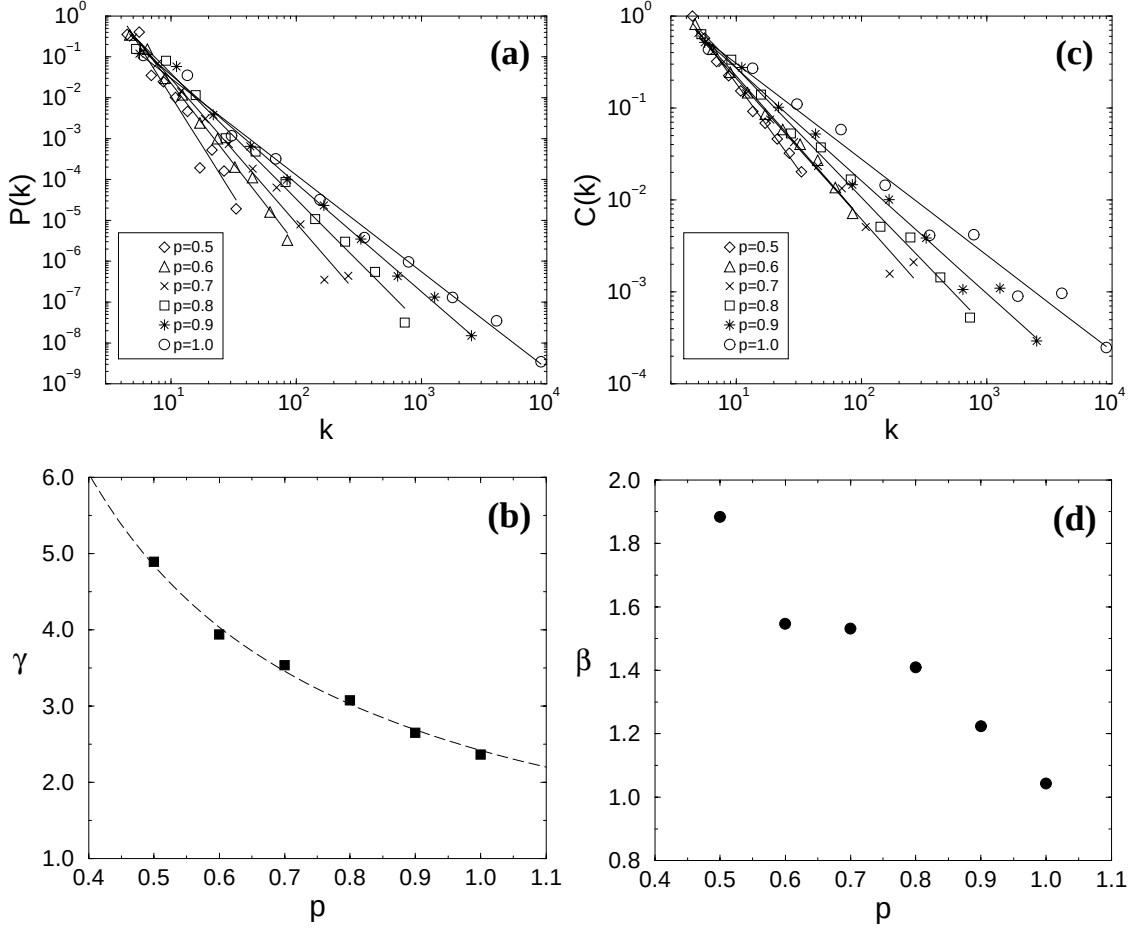
Figure 4.8. The scaling properties of the stochastic model. (a) The degree distribution for different p values, indicating that P(k) follows a power law with a p dependent slope. (b) The dependence of the degree exponent \gamma on p , determined by fitting power laws to the curves shown in (a) . The exponent \gamma appears to follow approximately \gamma(p) \sim 1/p (dashed line). (c) The C(k) curve for different p values, indicating that the hierarchical exponent \beta depends on p . (d) The dependence of \beta on the parameter p . The simulations were performed for N = 5^7(78,125) nodes.
