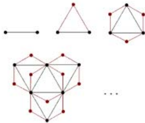
Figure 4.2. Construction of the pseudofractal network. (After [53])
