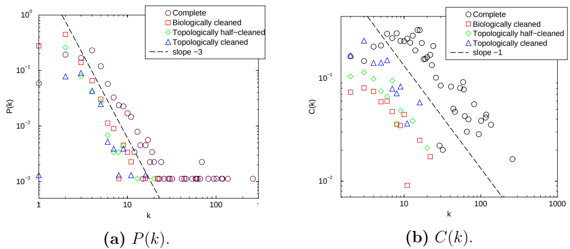
Figure 5.8. Degree distribution and clustering properties of all reduction stages of the E. coli metabolic network.
