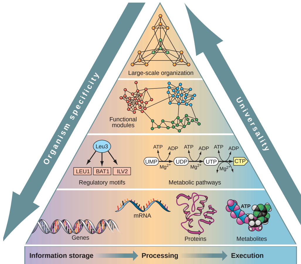
Figure 7.1. Life's complexity pyramid. (From [159])
