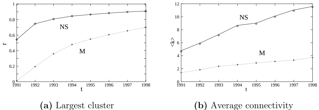
Figure 3.3. (a) Relative size of the largest cluster for the M and NS database. (b) Average number of links per node, \langle k \rangle . Results are computed on the cumulative data up to the given year.
