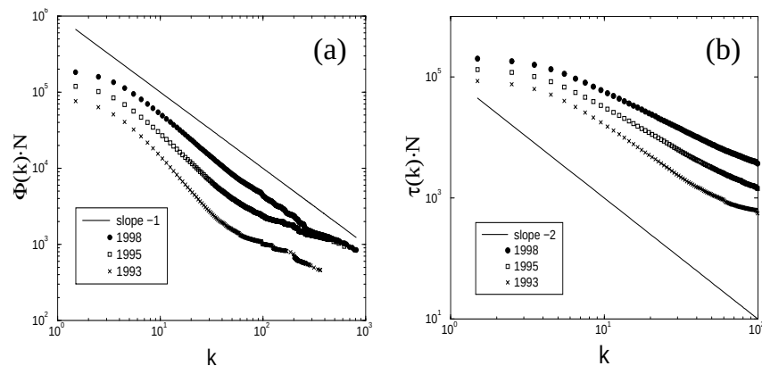
Figure 3.5. Scaling of \Phi(k) (a) and of \tau(k) (b) for the NS database, demonstrating the trends in the small and large k behavior of the degree distribution.
