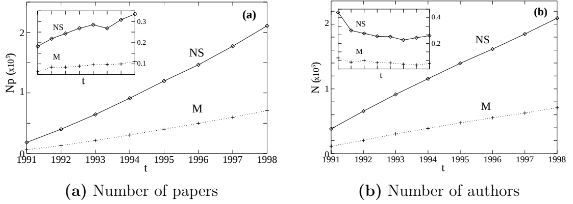
Figure 3.1. (a) Cumulative number of papers for the M and NS databases in the period 1991–98. The inset shows the number of papers published each year. (b) Cumulative number of authors (nodes) for the M and NS databases in the period 1991–98. The inset shows the number of new authors added each year.
