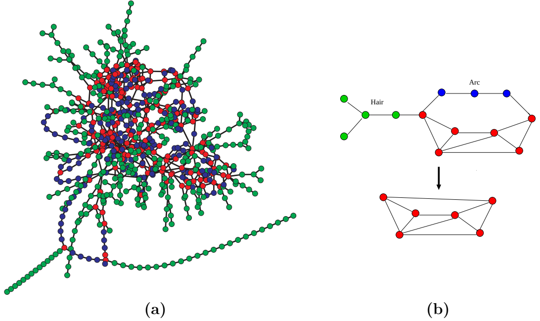
Figure 5.6. (a) The E. coli metabolic network after biochemical reduction. (b) Topological reduction, which implies temporally removing all hair (green), and replacing each arc (blue) with a single link.
