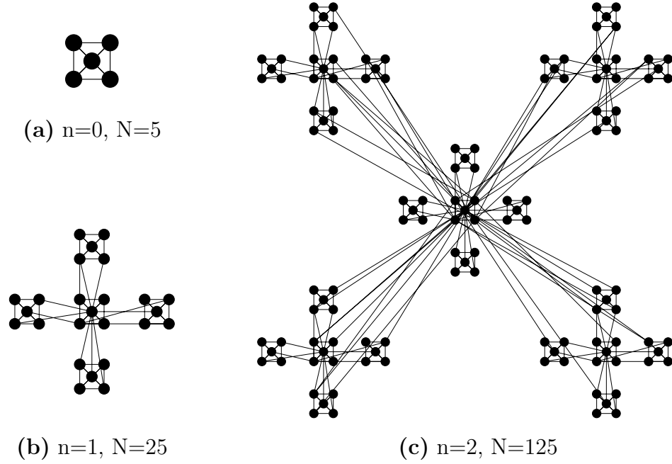
Figure 4.7. Iterative construction of the stochastic hierarchical network ( p = 3/5 ).
