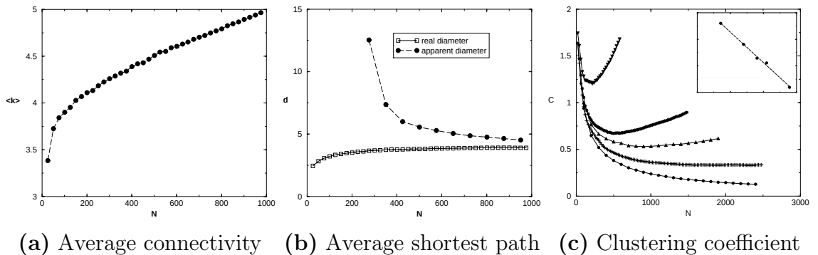
Figure 3.6. Computer simulated dynamics for N_{max} = 1000 , a = 0.001 , \beta = 1 and b = 2 . (a) Average connectivity. (b) Real and apparently measured average path length ( N_s = 200 ). (c) Clustering coefficient for different values of the a parameter as a function of the system size N (values of a are 0 ( \bullet ), 0.00025 (+), 0.0005 ( \Delta ), 0.00075 (*), and 0.002 ( \nabla )). The inset shows the scaling of the minimum value of C as a function of a , the line shows a fit \ln N_{min} = -(1.9 + 1.14 \cdot \ln a) .
