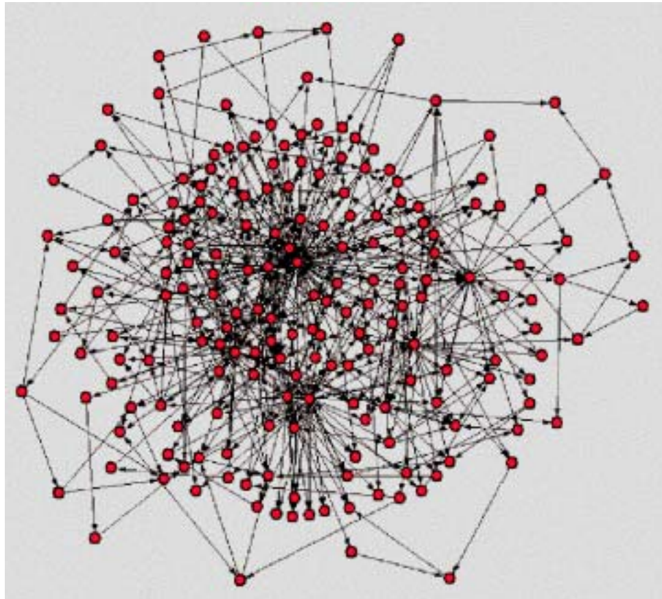
Figure 6.3. E. coli metabolic network based on similarity of reaction educts and products.
