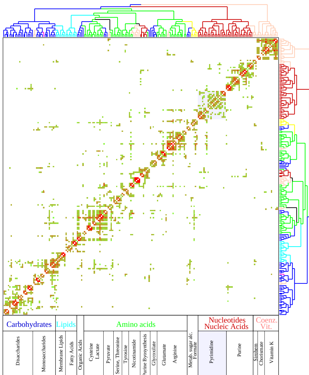
Figure 5.10. Topological overlap matrix corresponding to the E. coli metabolism, together with the corresponding hierarchical tree ( top and right side ) that quantifies the relationship between the different modules. The branches of the tree are color coded to reflect the functional classification of their substrates. The color code of the matrix denotes the degree of topological overlap shown in the matrix (See scale on Fig. 5.9a). On the bottom we show the large-scale functional map of the metabolism, as suggested by the hierarchical tree.
