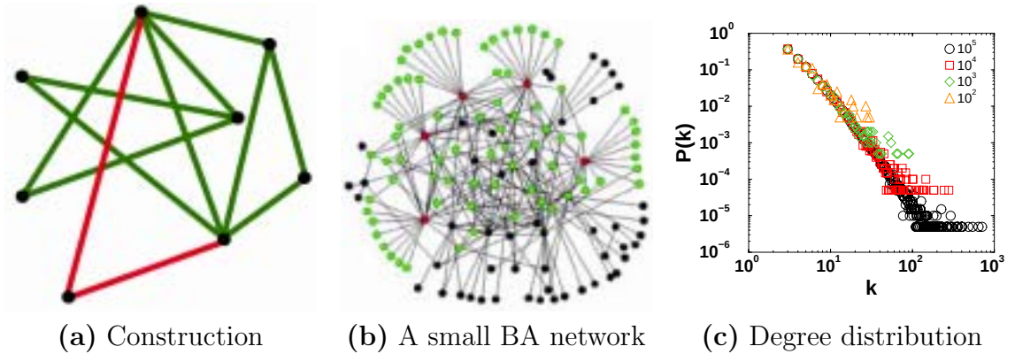
Figure 2.2. Barabási–Albert scale free network. (a) The model is constructed from m_0 initial nodes by subsequent addition of new nodes that connect to existing ones with probabilities proportional to their degree. (b) The scale free network generated by the BA model is not homogeneous, hubs with degrees orders of magnitude larger than the average coexist with many very low-connectivity nodes. (From [14]) (c) The P(k) degree distribution follows a power law, P(k) \sim k^{-\gamma} , with degree exponent \gamma = 3 .
