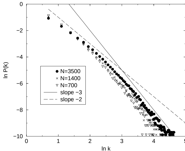
Figure 3.7. Connectivity distributions as predicted by numerical simulation for different stages of evolution of the network ( a = 0.001 , \beta = 1 and b = 2 ).
