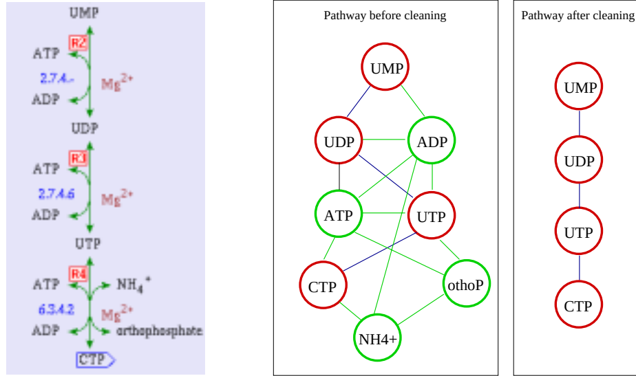
Figure 5.5. Biochemical reduction of the pathways of the metabolic network. The middle panel shows the full graph theoretic representation of the pathway shown in the left panel. The right panel displays the pathway after biochemical reduction.
