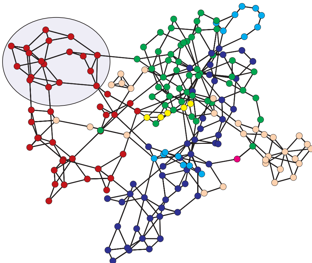
Figure 5.11. 3-D representation of the reduced E. coli metabolic network. Each node is color coded by the functional class to which it belongs, and is identical to the color code applied to the branches of the tree shown in figure 5.10. Note that the different functional classes are visibly segregated into topologically distinct regions of metabolism. The blue-shaded region denotes the nodes belonging to pyrimidine metabolism, discussed below.
