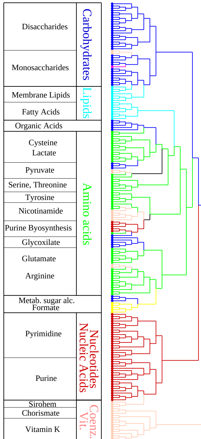
Figure 5.12. Hierarchical tree representing the reduced E. coli metabolic network.
