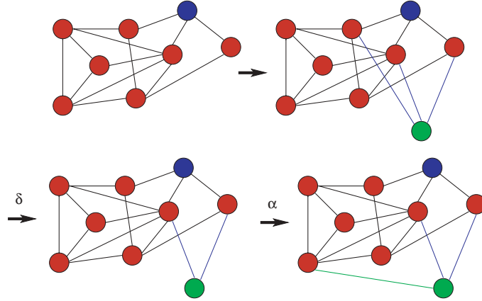
Figure 6.1. A duplication/diversification model for the evolution of protein interaction networks. A randomly chosen node (blue) is duplicated with all its interactions (green). Then these interactions may be lost with probability \delta , new ones can be gained with probability \alpha (green interaction).
