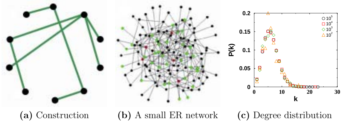
Figure 2.1. Erdős–Rényi random networks. (a) The model is constructed by laying down N nodes and connecting each pair of nodes with probability p . The figure shows a particular realization of such a network for N = 10 and p = 0.2 . (b) The random network generated by the Erdős–Rényi model is rather homogeneous, i.e. most nodes have approximately the same number of links. (From [14]) (c) The degree distribution P(k) is strongly peaked at k = \langle k \rangle and decays exponentially for large k .
