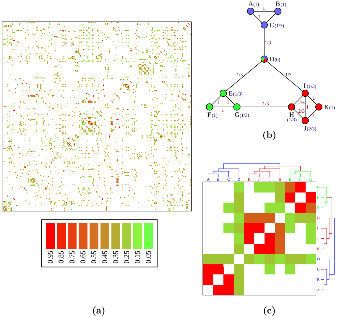
Figure 5.9. (a) Overlap matrix of alphabetical ordered substrates in the E. coli metabolic network. (b) Topological overlap illustrated on a small hypothetical network. On each link we indicate the topological overlap for the connected nodes and in parenthesis next to each node we indicate its clustering coefficient. (c) The topological overlap matrix corresponding to the small network shown in (b) . The rows and columns of the matrix were reordered by the UPGMA clustering method [191, 63], allowing us to identify and place close to each other those nodes that have high topological overlap. The matrix color code denotes the degree of topological overlap between the nodes (see side-bar on (a) ).
