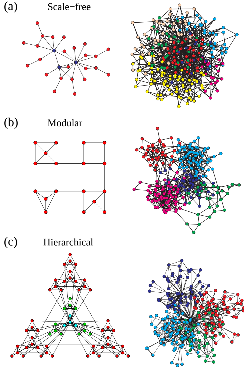
Figure 5.1. Complex network models. (a) Schematic illustration of a scale free network. (b) Schematic illustration of a manifestly modular network made of four highly interlinked modules connected to each other by a few links. (c) A hierarchical network with hierarchical levels represented in increasing order from blue to green to red. All 3D illustrations are networks with 256 nodes, arranged in space with a standard graph drawing algorithm [78].
