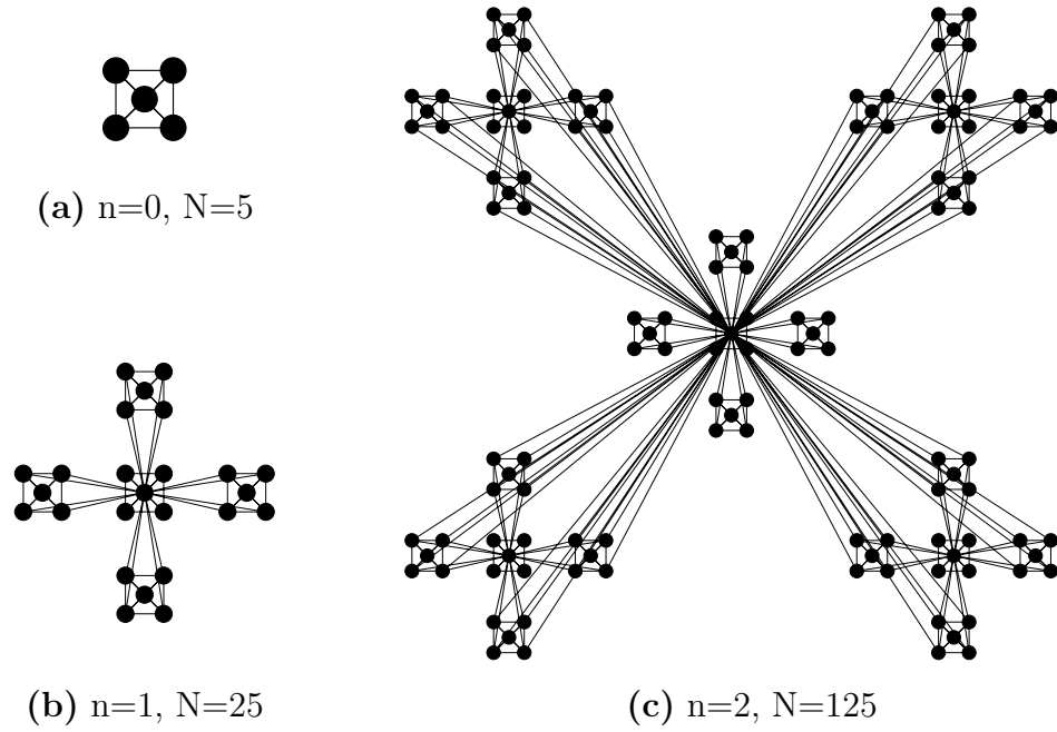
Figure 4.3. The iterative construction leading to a hierarchical network. Starting from a connected cluster of five nodes shown in (a) we create four identical replicas, connecting the peripheral nodes of each cluster to the central node of the original cluster, obtaining a network of N = 25 nodes (b) . In the next step we create four replicas of the obtained cluster, and connect the peripheral nodes again, as shown in (c) , to the central node of the original module, obtaining a N = 125 node network. This process can be continued indefinitely.
