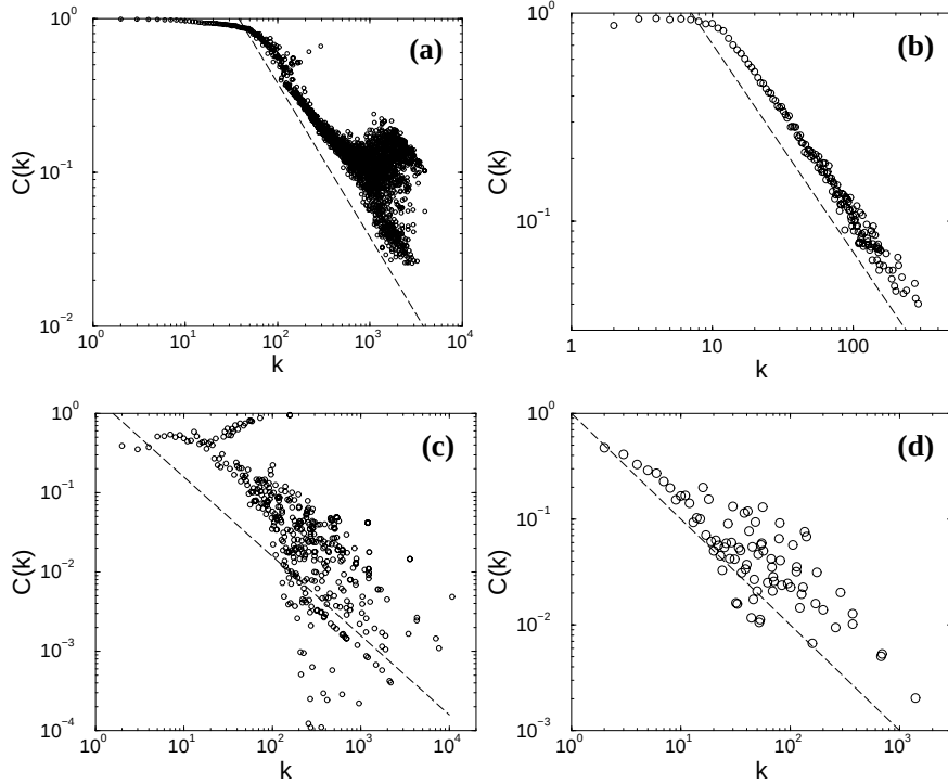
Figure 4.5. The scaling of C(k) with k for four large networks: (a) Actor network, two actors being connected if they acted in the same movie according to the www.IMDB.com database. (b) The semantic web, connecting two English words if they are listed as synonyms in the Merriam Webster dictionary [221]. (c) The World Wide Web, based on the data collected in Ref. [13]. (d) Internet at the Autonomous System level, each node representing a domain, connected if there is a communication link between them. The dashed line in each figure has slope -1 , following equation (4.8).
