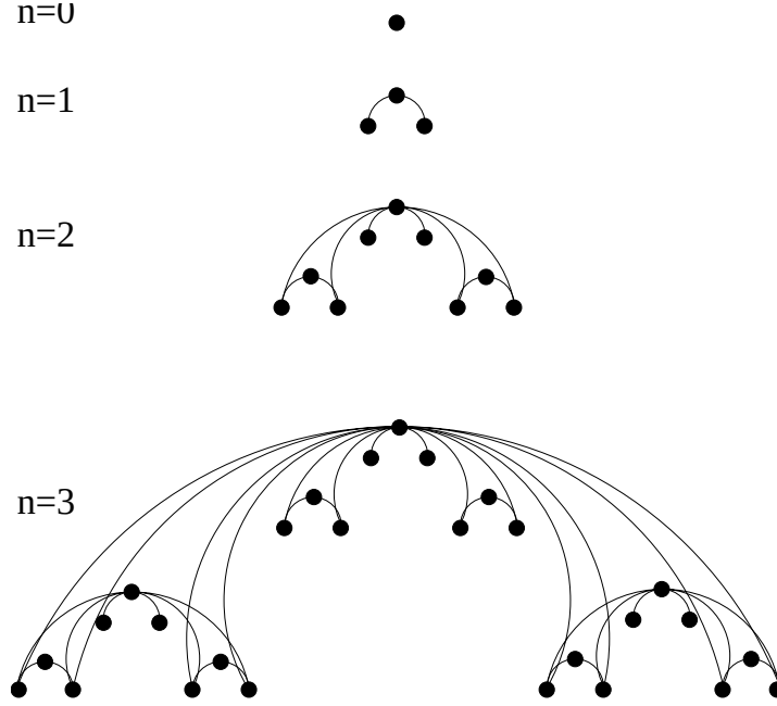
Figure 4.1. Construction of the deterministic scale free network.
