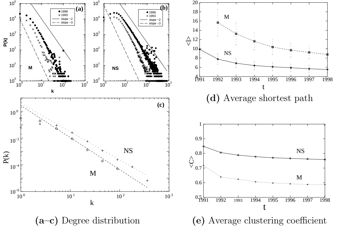
Figure 3.2. Degree distribution of the (a) M and (b) NS coauthorship networks, showing data based on the cumulative results up to years 1993 ( \times ) and 1998 ( \bullet ). (c) Degree distribution shown with logarithmic binning computed from the full dataset cumulative up to 1998. The lines correspond to the best fits, and have the slope 2.1 (NS, dotted) and 2.4 (M, dashed). (d) Average shortest path length in the M and NS databases. \langle l \rangle is computed on the cumulative data up to the indicated year. The error bars indicate the standard deviation of the distances between all pairs of nodes. (e) Clustering coefficient of the M and NS database, determined for the cumulative data up to the year indicated on the t axis.
