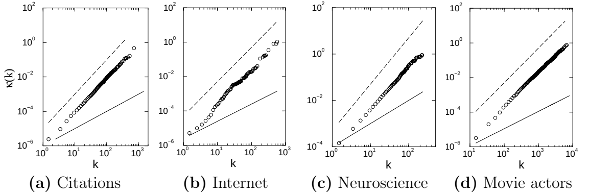
Figure 2.3. Measurement of the cumulative preferential attachment. Dashed line corresponds to linear preferential attachment, the continuous line to no preferential attachment. (From [99])
