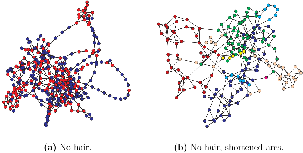
Figure 5.7. Topological reduction of the metabolic network. Starting from the biochemically reduced metabolic network shown in figure 5.6a, we removed all hair (a) and arcs (b) from the network. The color code of the nodes in the final figure denotes the corresponding substrate’s functional class (See Fig. 5.11).
