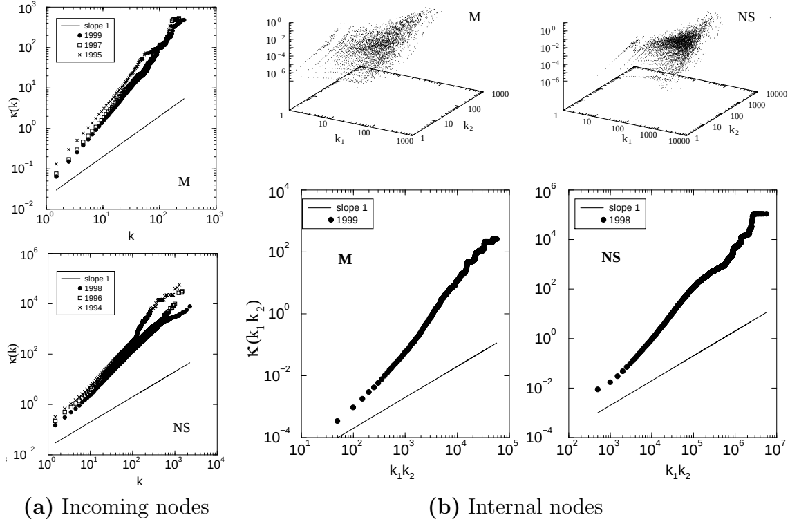
Figure 3.4. (a) Cumulative preferential attachment of newly added nodes, \kappa(k) . In the absence of preferential attachment \kappa(k) \sim k , shown as continuous line on the figures. (b) Internal preferential attachment \Pi(k_1, k_2) shown on the 3D plots (top); cumulative internal preferential attachment, \kappa(k_1 k_2) as a function of the k_1 k_2 product (bottom plots). The straight lines have slope 1, expected if there would be no preferential attachment. All results were computed by considering the new nodes coming in the specified year, and the network formed by nodes already present up to this year.
