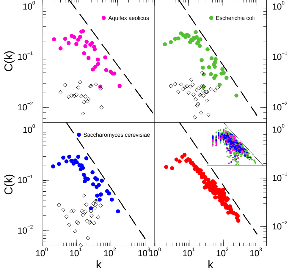
Figure 5.4. Dependence of the clustering coefficient on the node's degree in three organisms: (a) Aquifex aeolicus (archaea), (b) Escherichia coli (bacterium), (c) and Saccharomyces cerevisiae (eukaryote). In (d) the C(k) curves averaged over all 43 organisms are shown, while the inset displays all 43 species together. The dashed lines correspond to C(k) \sim k^{-1} , and in (a–c) the diamonds represent C(k) expected for a scale free network (Fig. 5.2a) of similar size, indicating the absence of scaling. The wide fluctuations are due to the small size of the network.
